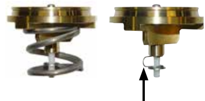
Blocking clip (check valve blocked)
