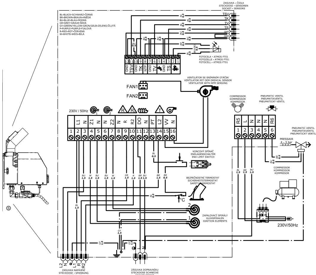
21-06-01_A25-COMPACT_6P_AC07X-C_PNEU - FT01
