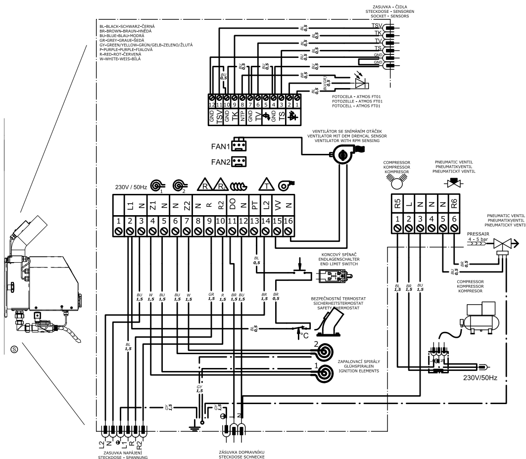
21-06-01_A25-COMPACT_6P_AC07X-C_PNEU - FT01
